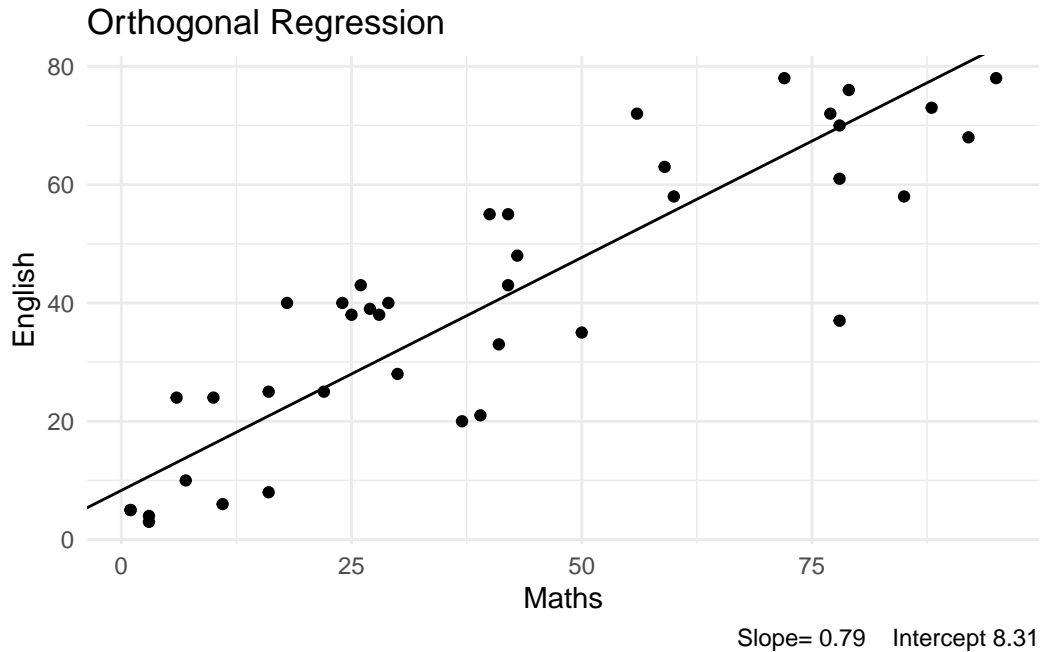
Figure 5.1: Orthogonal regression
