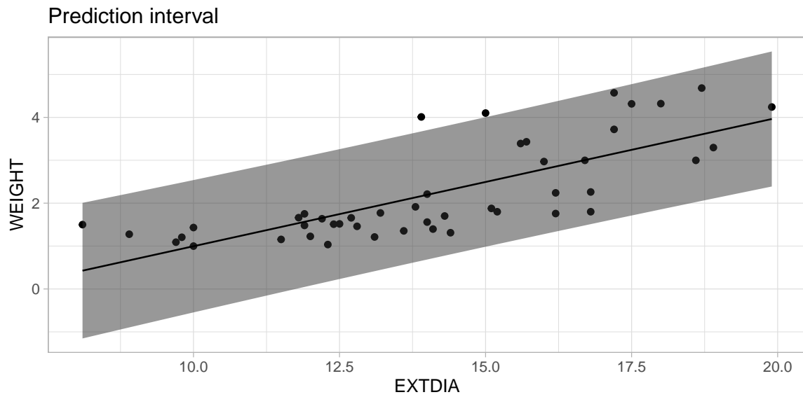
Figure 2.4: Confidence intervals and prediction intervals
